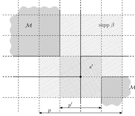
FIGURE 11. If the coefficient graph of a basis function \beta has two connected components, then shrinking \text{supp } \beta (single hatching) gives a cube s' (double hatching) that touches the boundary of \mathcal{M} (solid light gray) in at least two disjoint sets of points. The center of s' (black dot) belongs to a self-intersection of a certain offset (thick solid black line).
