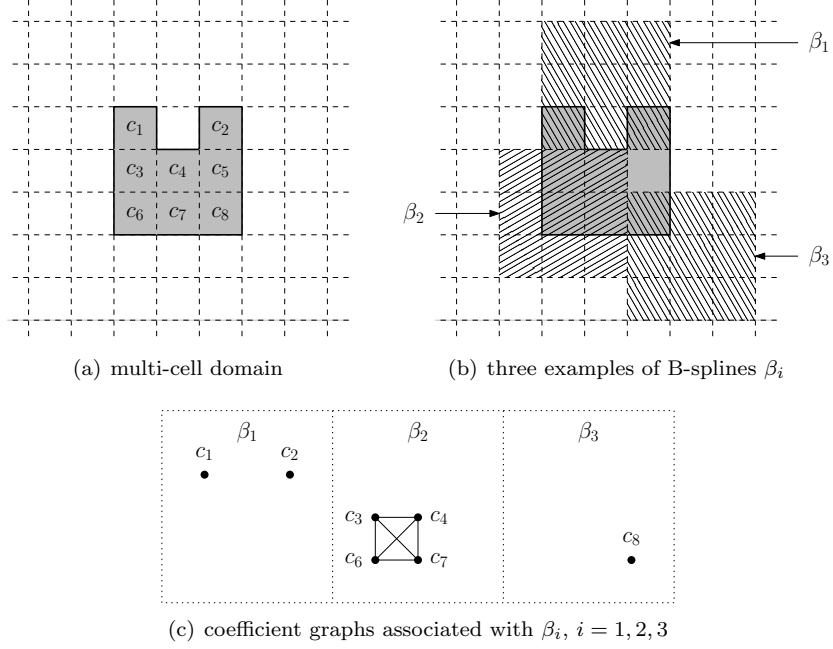
FIGURE 3. A multi-cell domain with eight cells (a), the supports of three biquadratic B-splines (b) and the associated coefficient graphs (c).
