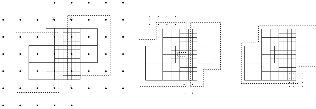
Figure 9: Multi-level mesh with bi-quartic basis functions. The thick dashed line represents the offset at distance 3/4 . From left to right:: TDHB-splines from \hat{\mathbf{G}}_B^0, \hat{\mathbf{G}}_B^1, \hat{\mathbf{G}}_B^2 . Note that the offset condition would not be satisfied for larger degrees.
