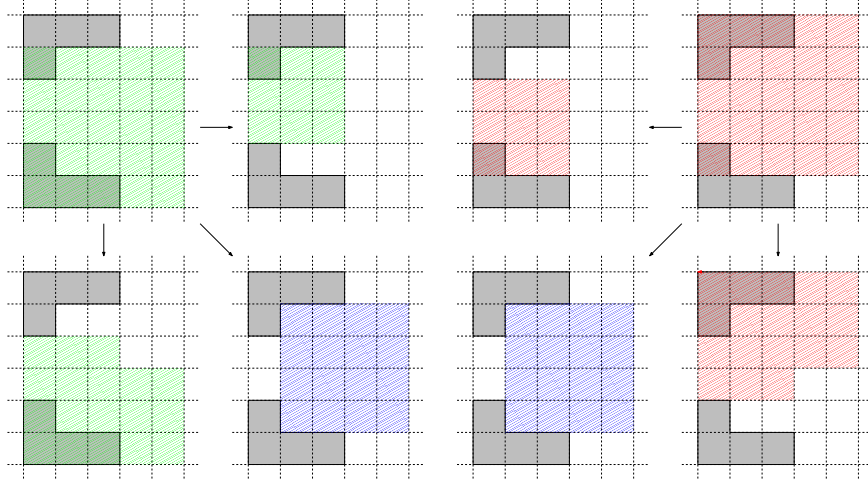
Figure 3: Decoupling bi-quartic B-splines with single knots and dyadic refinement. The ring \Delta^\ell is shown in gray. The hatched regions are supports of functions from \mathbf{G}^\ell and \hat{\mathbf{G}}^\ell , the arrows show the decoupling. The two functions in the top left and top right are decoupled into 2 larger functions and 16 B-splines (corresponding to isolated vertices of the coefficient graph) each.
