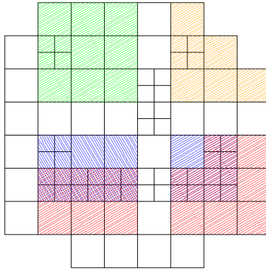
Figure 6: Mesh with biquadratic decoupled B-splines. The support of a basis function (provided that it is sufficiently far away from the boundary of \Omega ) consists of 3 \times 3 cells. The function may split into up to 4 decoupled functions. In the example, the functions either split into two functions (pairs of red and blue supports with purple overlap) or remain unchanged (green supports). The shape of the support of the upper right function (orange) is caused by the intersection with the domain boundary.
