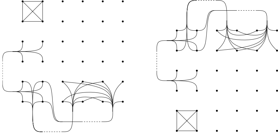
Figure 4: The decoupling graphs of the functions from Figure 3.
