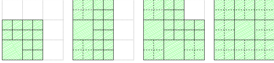
Figure 5: Possible shapes of supports of decoupled biquadratic spline functions, up to rotations and symmetries, depending on the local shape of the mesh in the support. Here we assume that there are no intersections with the boundary of the domain \Omega . The larger cells belong to level \ell , whereas the smaller ones to level \ell + 1 . The dotted lines indicate the size of the support before decoupling, whereas the dashed lines may or may not be present as long as the mesh does not reduce to a case with a smaller support. Note that due to (2) the supports near to domain boundary could be trimmed, see the figure below.
