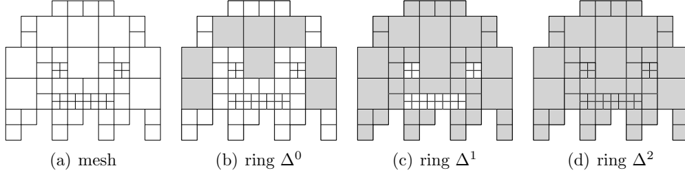
Figure 2: An example of a hierarchical mesh and the associated rings.
