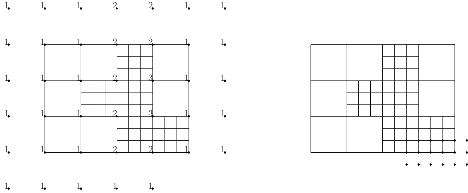
Figure 7: Bicubic B-splines from \mathbf{G}_B^0 and \mathbf{G}_B^1 . Left: dots are placed in the Greville points corresponding to functions from \mathbf{G}_B^0 and the numbers indicates in how many functions from \hat{\mathbf{G}}_B^0 will the particular function be decoupled into. Right: functions from \mathbf{G}_B^1 .
