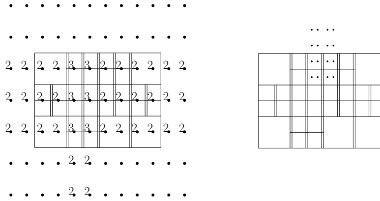
Figure 8: Bivariate B-splines with \mathbf{p}^\ell = (5,4) and \mathbf{m}^\ell = (2,1) . Left: dots depict the Greville points functions from \mathbf{G}_B^0 ; those that decouple into more than function have also assigned the number of decouple functions derived from them. Right: B-splines from \mathbf{G}_B^1 , which are also present in \mathcal{T} .
