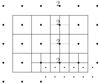
Figure 10: Biquadratic splines. Thick dots correspond to Greville points from \mathbf{G}_B^0 , the smaller dots to functions from \mathbf{G}_B^1 . If a number is present at a dot, it specifies the number of functions that this function decouples into (note that the functions from the finest level do not get decoupled). The dotted lines represent the “passive” edges, i.e., the edges that could be omitted without changing the dimension of the spline space.
